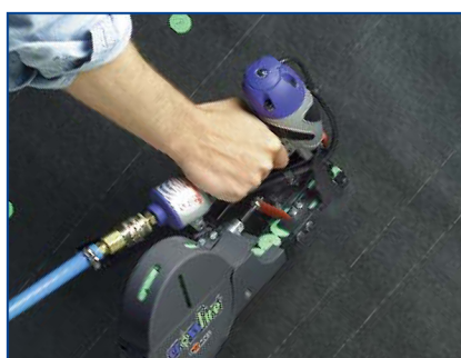
Roofing Felt
